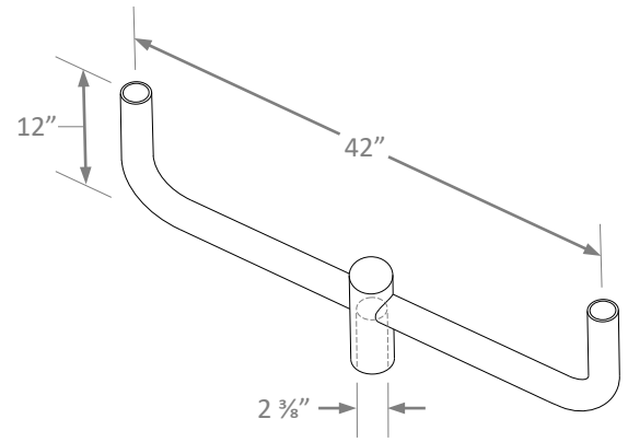
Double Bullhorn 180° Mounting Bracket PN: D180BH Bullhorn requires slip-fitter mount
