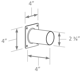
Wall Mount Bracket PN: WMB
