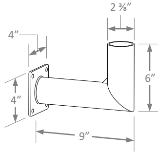
90° Wall Mount Bracket PN: WMB90
